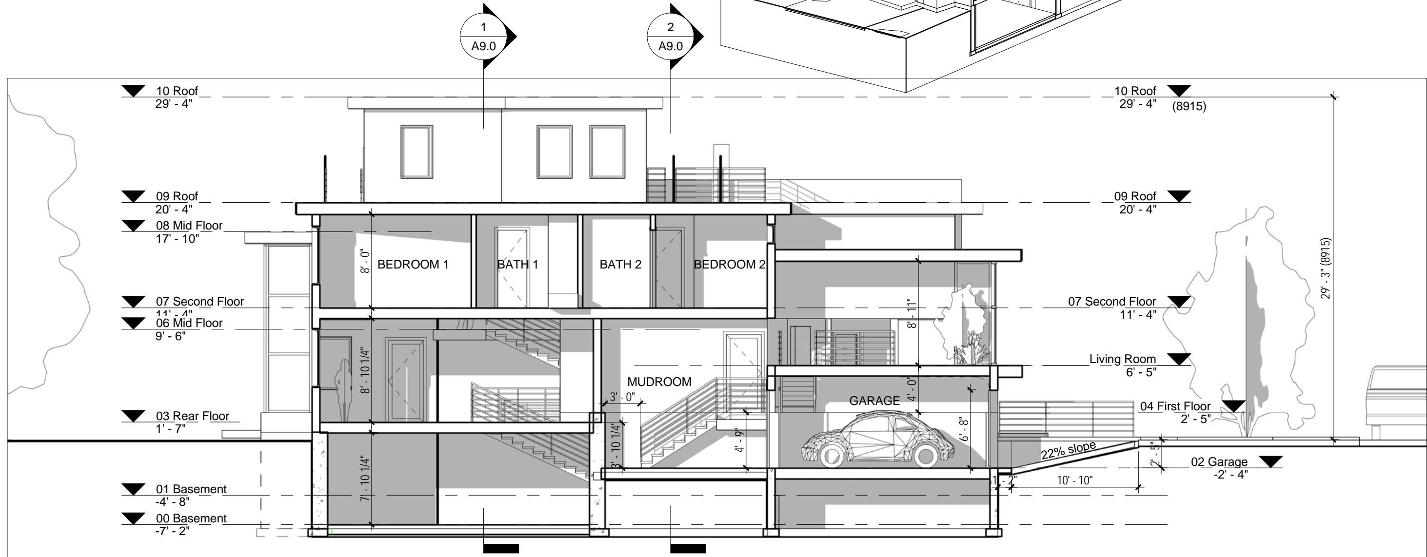
1 Section A 1/8" = 1'-0"
