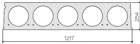
254mm slab
