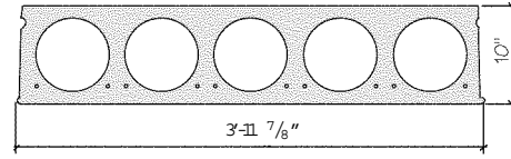
10" slab
