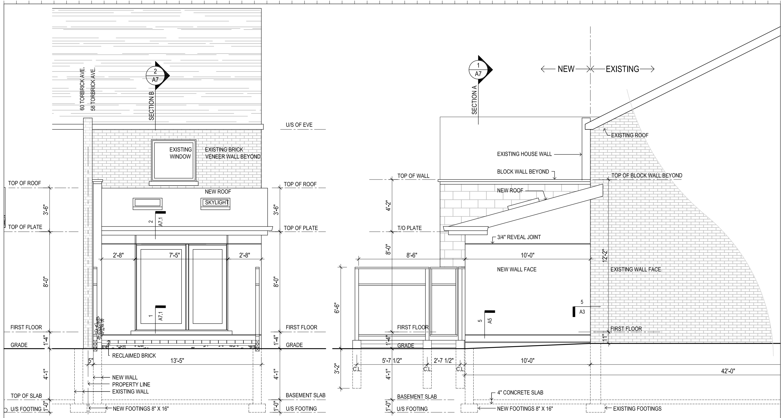
2 North Elevation Scale: 1/4"=1'-0"
