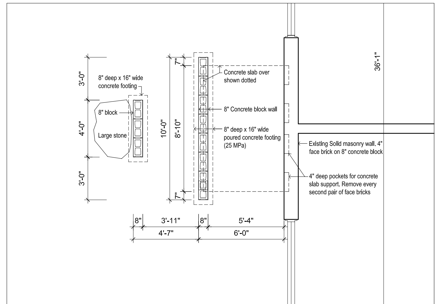
1 A2 Foundation Plan Scale: 1/4" = 1'-0"
