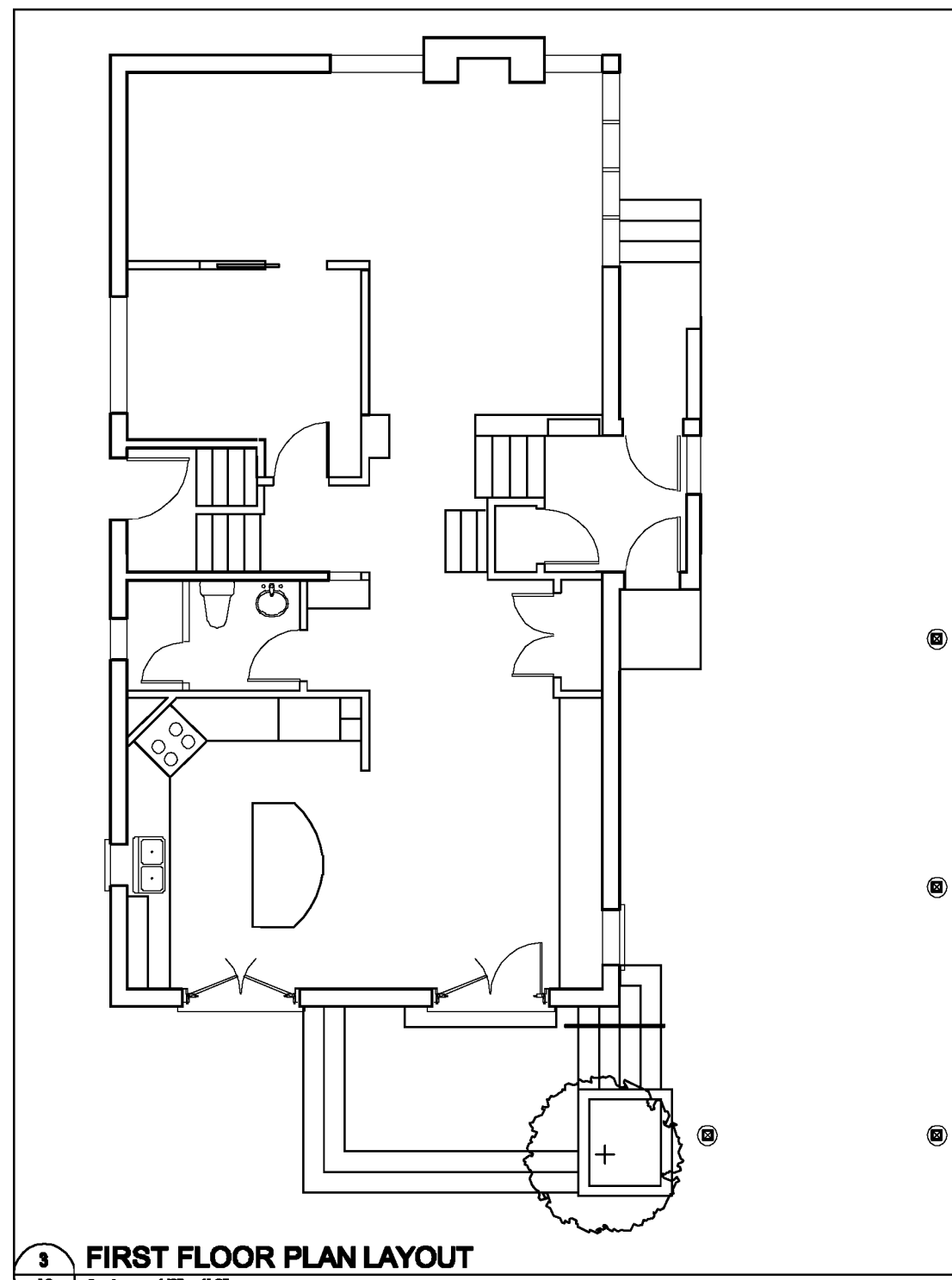
2 FIRST FLOOR PLAN REMOVALS A3 Scale: 1/8" = 1'-0"
