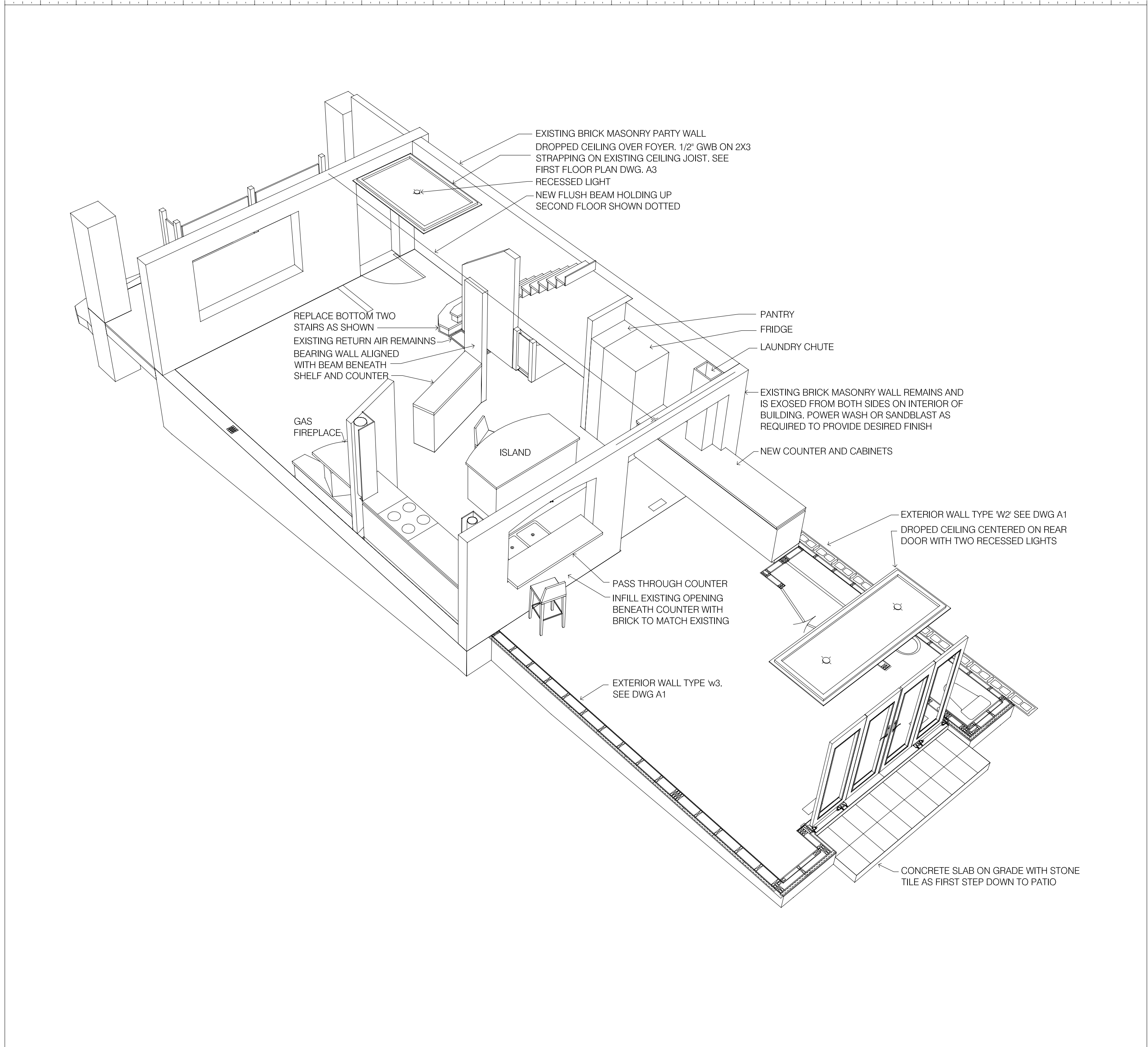
3D VIEW TOWARD FIRST FLOOR
